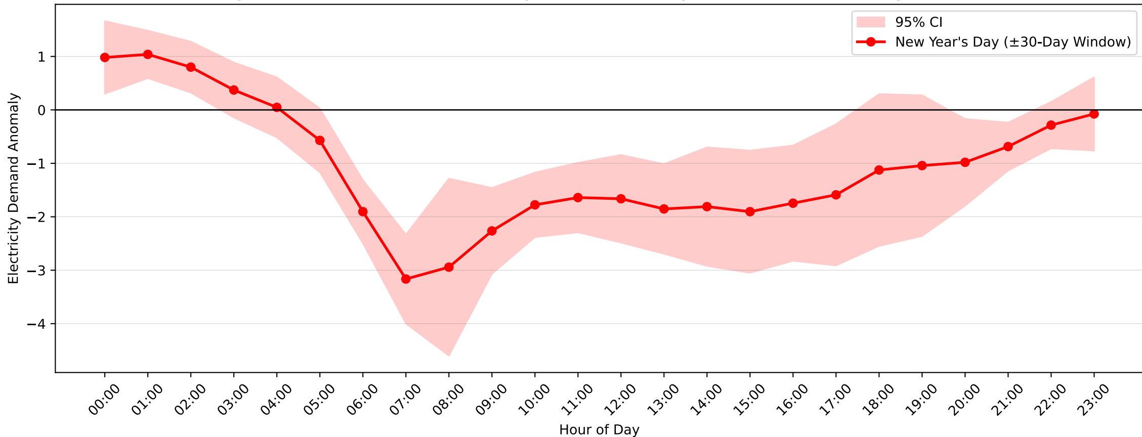
Balgowlah North Demand Anomaly: New Year's Day (2013-2014, \pm 30 -Day Window)
