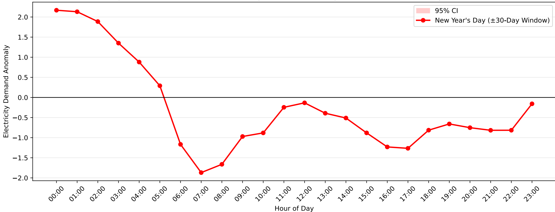
Balgowlah North Demand Anomaly: New Year's Day (2017-2018, \pm 30 -Day Window)
