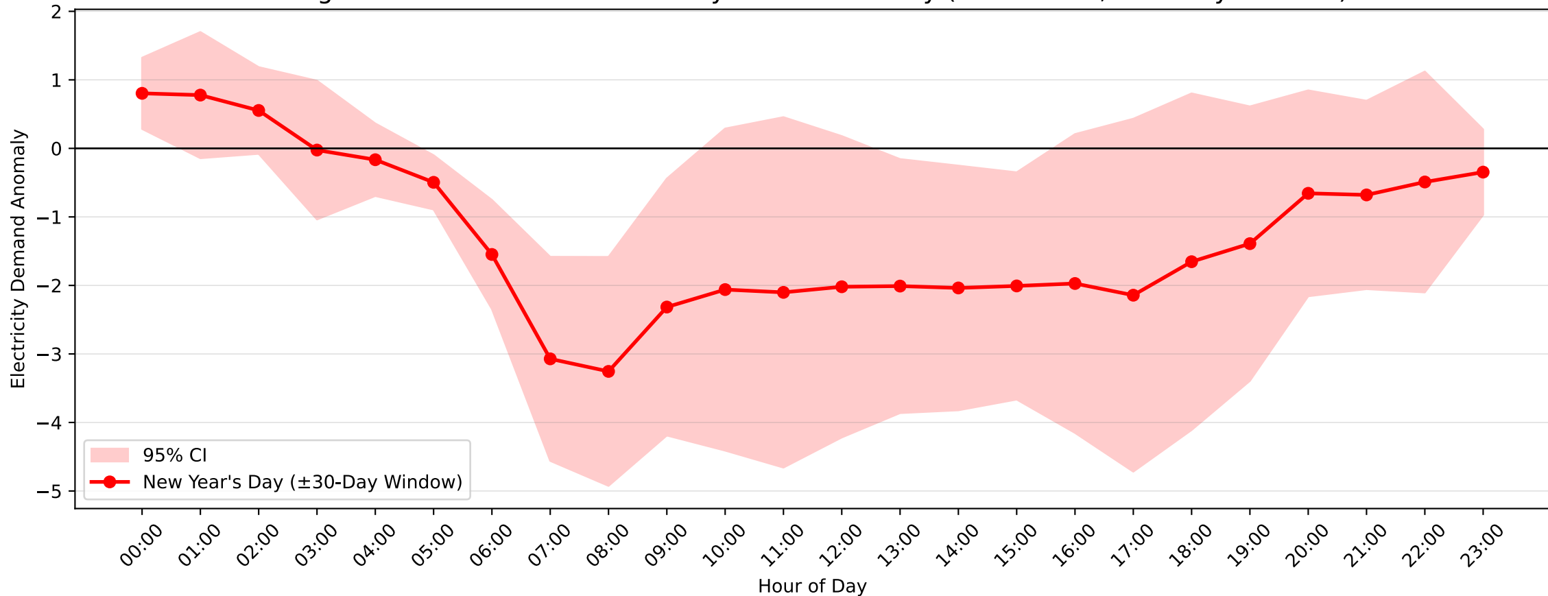
Balgowlah North Demand Anomaly: New Year's Day (2012-2013, \pm 30 -Day Window)
