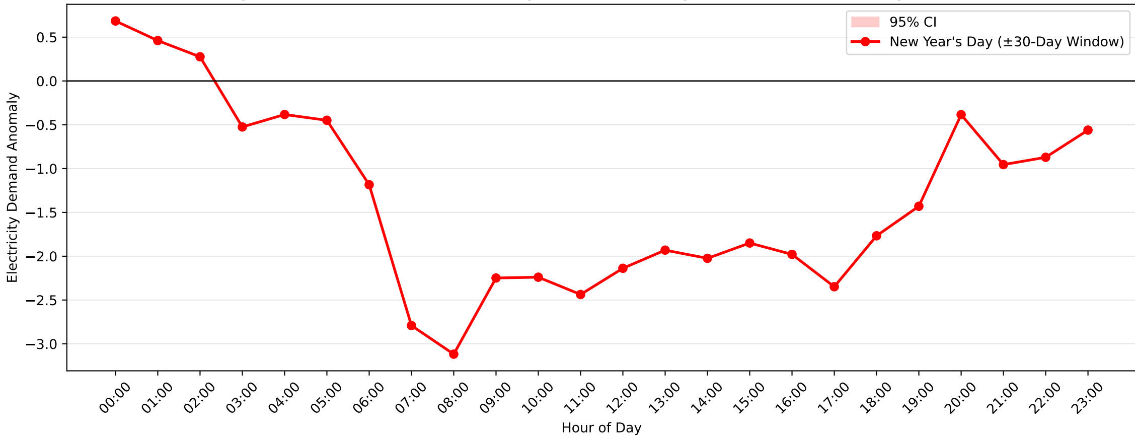
Balgowlah North Demand Anomaly: New Year's Day (2011-2012, \pm 30 -Day Window)
